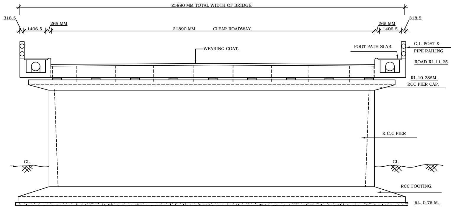
CROSS SECTION
