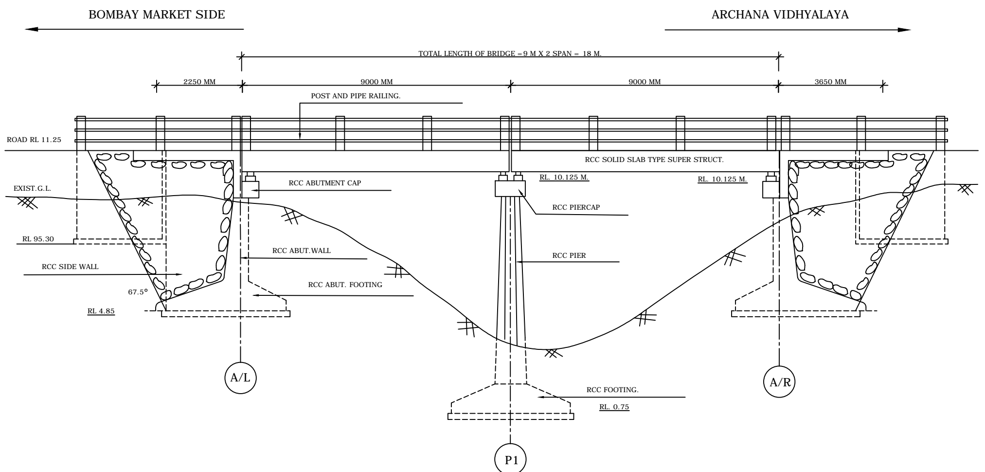
SECTIONAL ELEVATION
