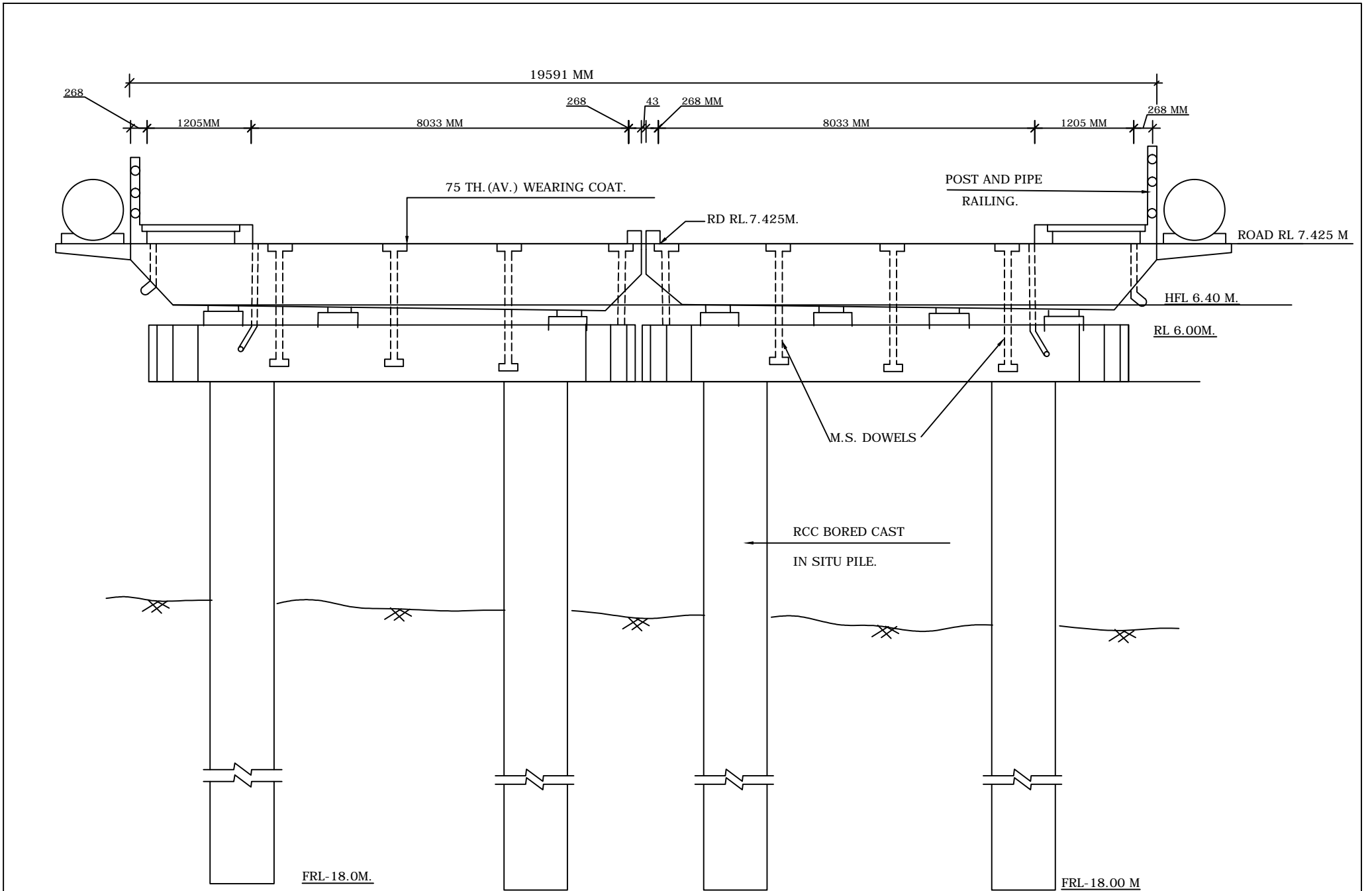
CROSS SECTION
