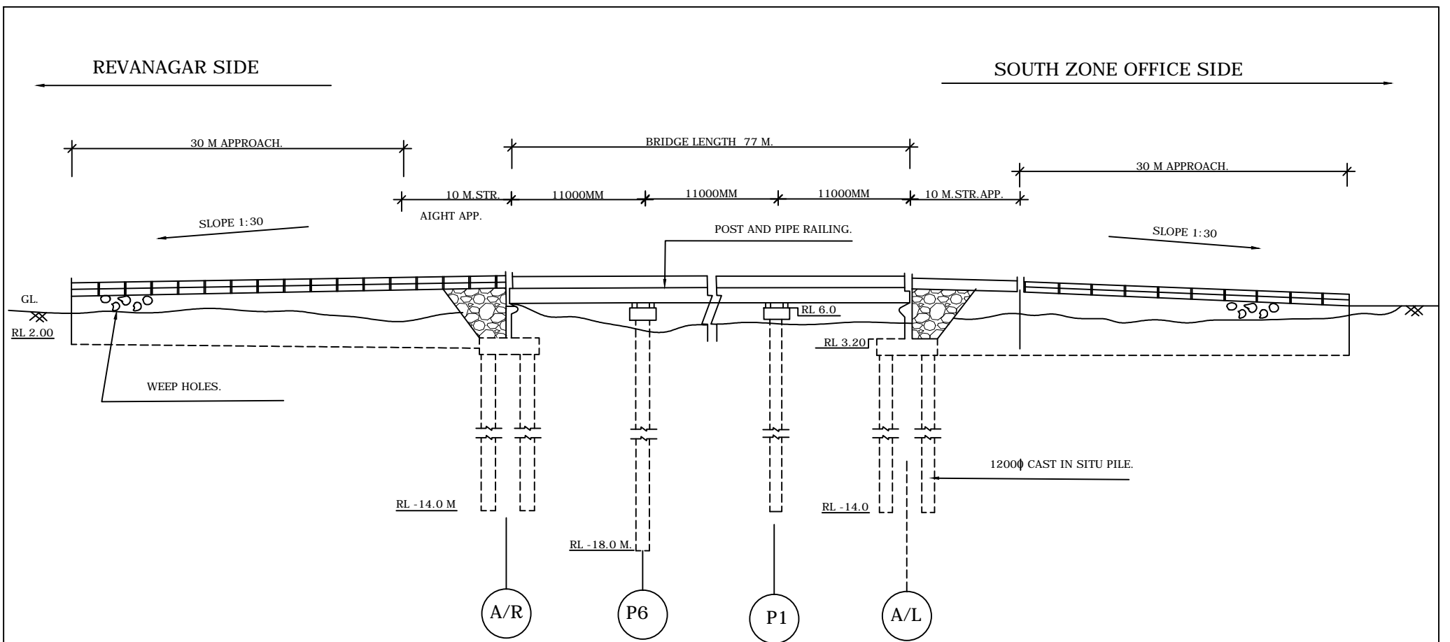
SECTIONAL ELEVATION
